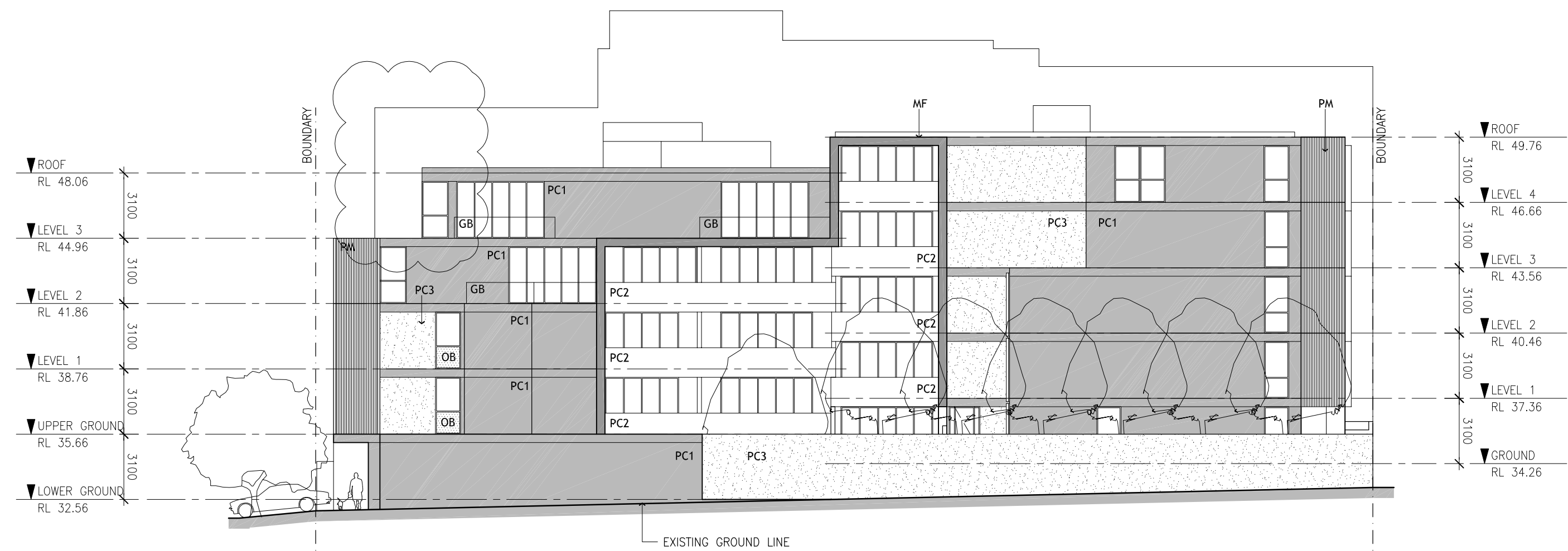
EAST ELEVATION
