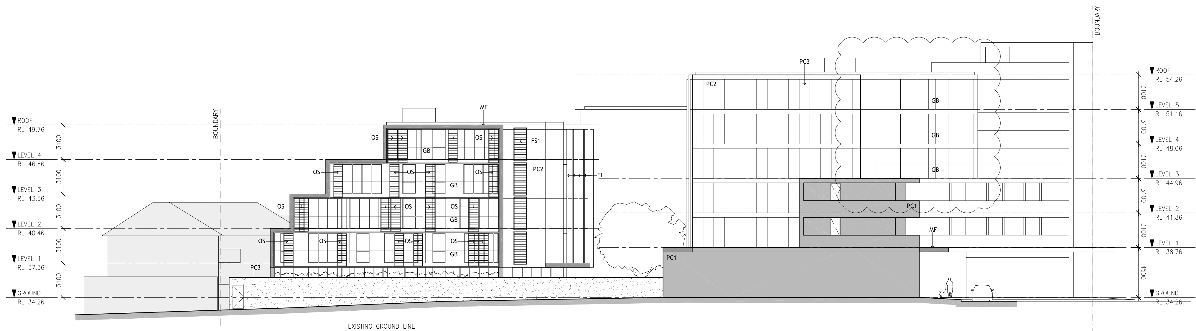
NORTH ELEVATION
