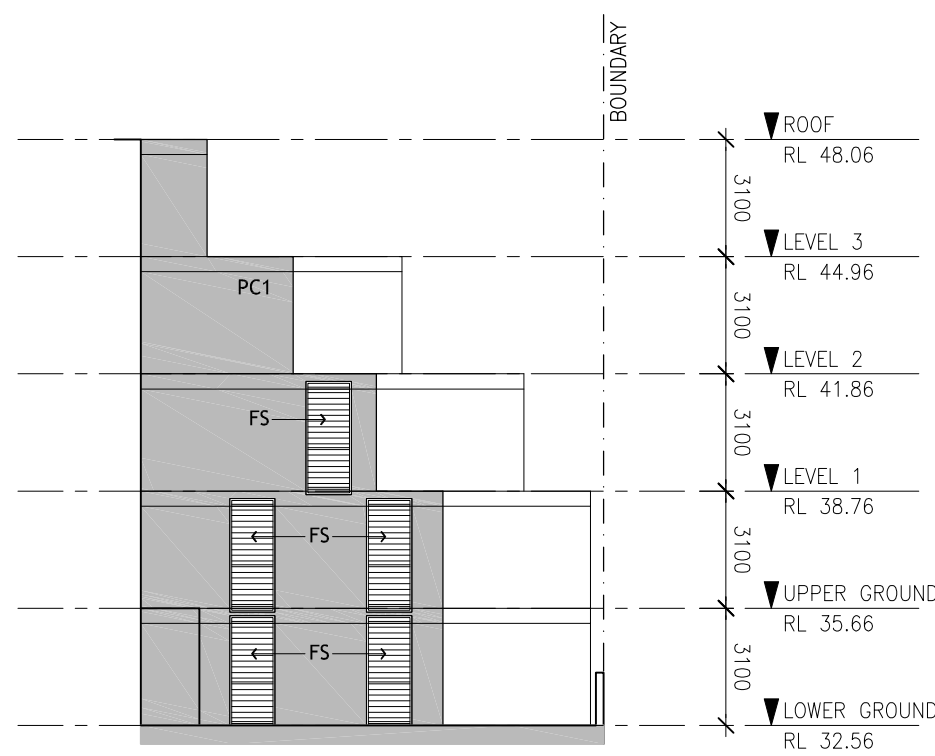
SOUTH ELEVATION (PART)
